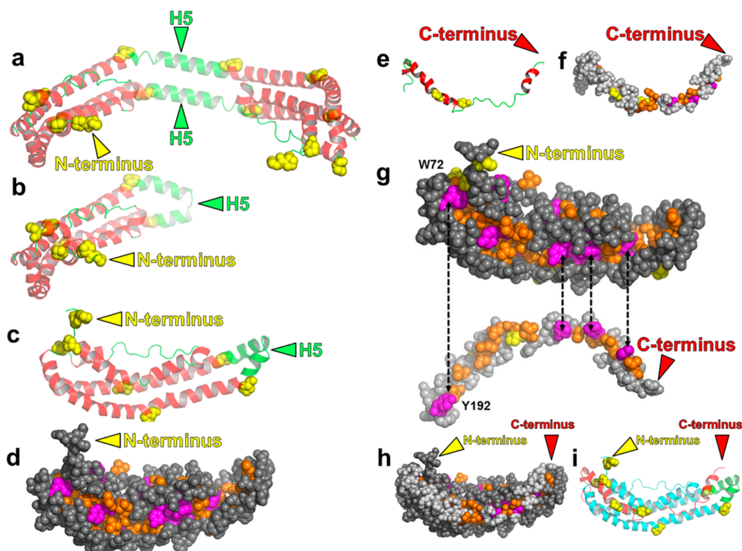
Figure 1. Creation of a lipid-free apoA-I monomer model from a combination of the C-terminally truncated (Δ185–243)apoA-I 26 and N-terminally truncated (Δ1–43)apoA-I 17 crystal structures. (a and b) Depth-cued ribbon images showing the creation of a monomer from the crystal structure of the (Δ185–243)apoA-I dimer of Mei and Atkinson. 26 (a) crystal dimer 26 and (b) monomeric (Δ185–243)apoA-I created by forming a hairpin from H5. Because residues 1 and 2 were missing from the crystal structure, they were added from a previous MD simulation. (c–i) Development of the initial crystal model. Color codes for ribbon models: H5, green; other helical domains, red; nonhelical domains, green; prolines in panels a–c, e–g, and i, space-filling yellow. Color codes for space-filling models: aromatic residues, magenta; nonaromatic hydrophobic residues, gold; prolines, yellow. (c) Reorientation of the ribbon model of the (Δ185–243)apoA-I monomer in panel b. (d) Space-filling model of the structure in panel c showing its deep hydrophobic cleft. (e) Ribbon model of residues 183–243 from the N-terminally truncated crystal structure. 17 (f) Space-filling model of the structure in panel e. (g) Alignment of aromatic and hydrophobic residues between the (Δ185–243)apoA-I monomer model (1–182) and the N-terminally truncated fragment. (h) Initial crystal model (space-filling) for the full-length monomer. (i) Ribbon model of the structure in panel h. Residues 1–182 are colored cyan and residues 183–243 red.
